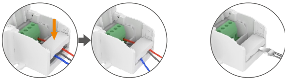
Push the tension plate down to fix the electric wires.
